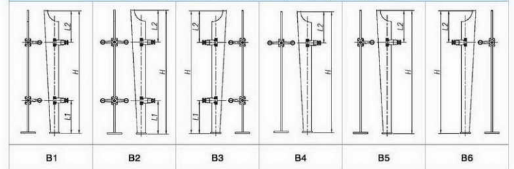
联接件结构图和顺序号 Balustrade Bracket structure drawing with sequence number
