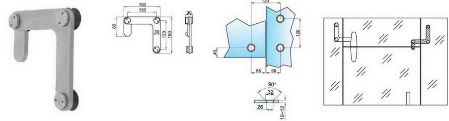
L fixing connector with door stopper
