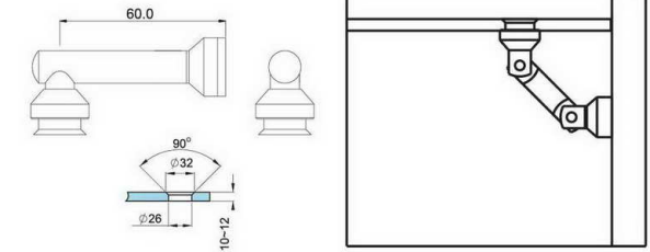
glass fixing connector wall to glass, both side angle adjustable
