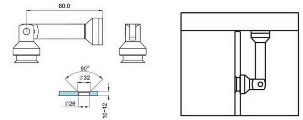
glass fixing connector wall to glass, one side angle adjustable
