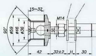
TC32(原代号Original Code:TC42)
