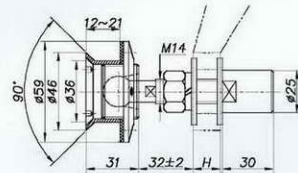
TC31(原代号Original Code:TC43)
